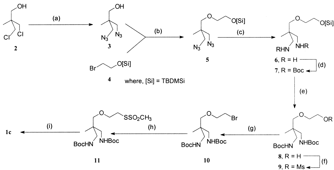
Scheme 2. (a) \text{NaN}_3 , 130^\circ\text{C} , 98%; (b) \text{NaH} , \text{Bu}_4\text{NI} , THF then 4 , 55%; (c) \text{H}_2 , Pd-black, MeOH; (d) \text{Boc}_2\text{O} , \text{NaOH}(\text{aq})/\text{dioxan} , 72% over 2 steps; (e) TBAF, THF, 93%; (f) \text{MsCl} , \text{Et}_3\text{N} , \text{CH}_2\text{Cl}_2 , 99%; (g) \text{LiBr} , acetone, \Delta , 93%; (h) \text{NaSSO}_2\text{CH}_3 , DMF, 50^\circ\text{C} , 87%; (i) \text{CF}_3\text{COOH} , \text{CH}_2\text{Cl}_2 , then ion exchange chromatography, 67%.
